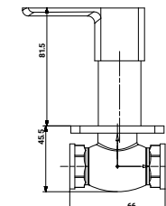
SG-3008CC Concealed Stop Cock Adjustable Wall Flange (15mm) with Brass Handel & Flange
