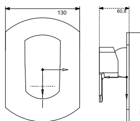
SG-3036SPK4 Exposed Part Kit of Shower or Spout Single Lever Diverter with Brass Handel & Flange
