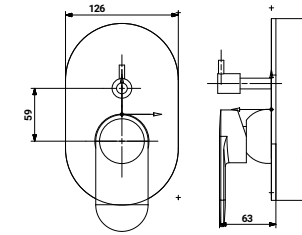
ST-3137SPK2 Exposed Part Kit of 5 Ways Single Lever Diverter with Brass Handel & Flange
