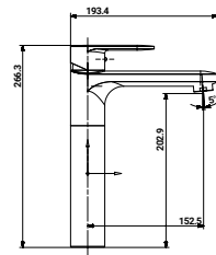
ST-3127SBML Single Lever Basin Mixture with 450mm Tube Exten. Body with Brass Handel & Flange
