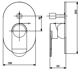
ST-3128SPK2 Exposed Part Kit of Single Leaver Hi/Flow Diverter 45MM with Brass Handel & Flange
