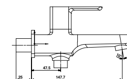
SG-3007BC2 Bib Cock with Brass Handel & Flange (Single Handel)
