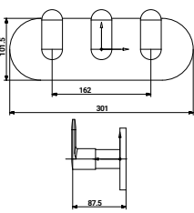
ST-3131DV4 Exposed Part Kit of 4 Way Diverter with Brass Handel & Flange
