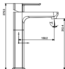
SG-3027SBML Single Lever Basin Mixture with 450mm Tube Exten. Body with Brass Handel & Flange
