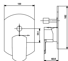
SG-3028SPK2 Exposed Part Kit of Single Leaver Hi/Flow Diverter 45MM with Brass Handel & Flange
