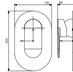
ST-3136SPK4 Exposed Part Kit of Shower or Spout Single Lever Diverter with Brass Handel & Flange
