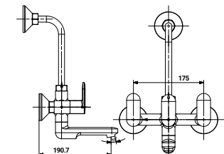
ST-3115WM Wall Mixture with Provision For Over Head Shower with Bend
