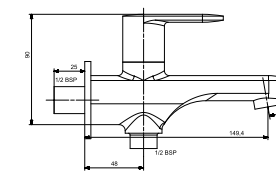
ST-3107BC2 Bib Cock with Brass Handel & Flange (Single Handle)
