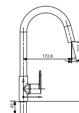
ST-3110SNL Swan Neck Extension Spout with Brass Handel & Flange
