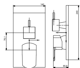
SG-3035SJM Exposed Part Kit of Jet Single Lever 3 Way Diverter (20MM)
