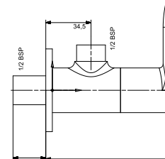
ST-3105AV Angle Valve with Brass Handel & Flange
