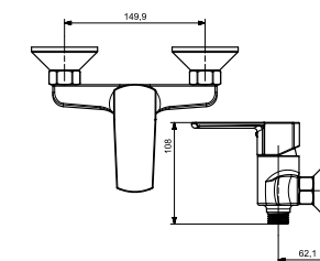
SG-3041SWM Single Lever Wall Mixture with Only Connection Pipe Provision (Wall Mounted) with Brass Handel & Flange
