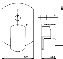
SG-3033SPK3 Exposed Part Kit of Single Lever Hi/Flow Diverter 40MM with Brass Handel & Flange
