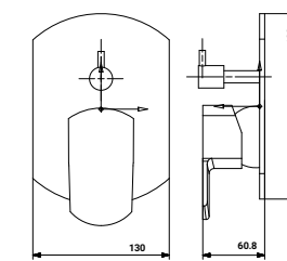
SG-3037SPK2 Exposed Part Kit of 5 Ways Single Lever Diverter with Brass Handel & Flange
