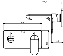
ST-3119SPK Exposed Part Kit of Sink Mixture Wall Mounted Swing Spout with Brass Handel & Flange
