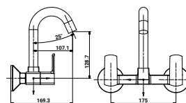
SG-3023SM Sink Mixture Wall Mounted Swing Spout with Brass Handel & Flange
