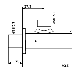
SG-3005AV Angle Valve with Brass Handel & Flange
