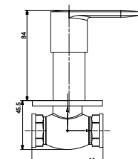
ST-3108CC Concealed Stop Cock Adjustable Wall Flange (15mm) with Brass Handel & Flange
