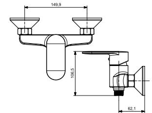
ST-3141SWM Single Lever Wall Mixture with Only Connection Pipe Provision (Wall Mounted) with Brass Handel & Flange
