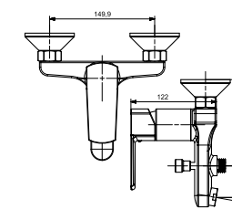
SG-3039SWM Single Lever Wall Mixture with Provision Hand Shower (Wall Mounted) with Brass Handel & Flange
