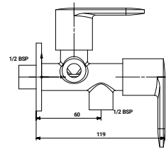
ST-3123SM Sink Mixture Wall Mounted Swing Spout with Brass Handel & Flange
