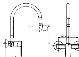
SG-3040SSM Single Lever Sink Mixture with Swinging Spout (Wall Mounted) with Brass Handel & Flange
