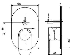
ST-3133SPK3 Exposed Part Kit of Single Lever Hi/Flow Diverter 40MM with Brass Handel & Flange
