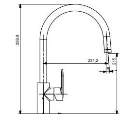
ST-3132SSM Single Lever Sink Mixture Side Handle 450mm Braided Hose (table mounted) with Brass Handel & Flange
