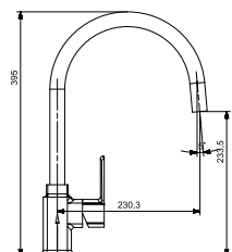
SG-3032SSM Single Lever Sink Mixture Side Handle 450mm Braided Hose (Table Mounted) with Brass Handel & Flange
