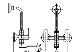
SG-3015WM Wall Mixture with Provision For Over Head Shower with Bend
