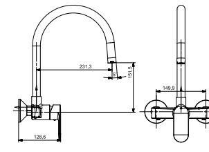
ST-3140SSM Single Lever Sink Mixture with Swinging Spout (Wall Mounted) with Brass Handel & Flange
