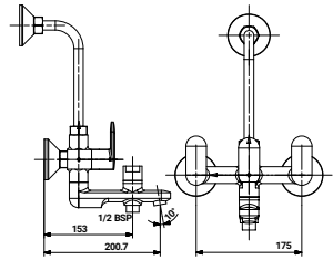
ST-3117WM3 Wall Mixture 3 in 1 with Provision for Over Head Shower with Brass Handel & Flange
