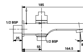
SG-116BTS2 Bath Tub Spout Attached with Brass Flange
