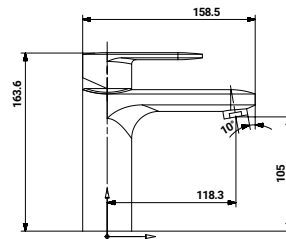
ST-3126SBM Single Lever Basin Mixture with 450mm Tube with Brass Handel & Flange
