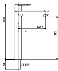
ST-3129PCL2 Pillar Cock Extension Body 10" with Brass Handel & Flange
