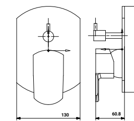
SG-3038SPK2 Exposed Part Kit of Single Leaver Hi/Flow Diverter 45MM with Brass Handel & Flange
