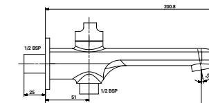
ST-118BTS2 Bath Tub Spout Attached with Brass Flange
