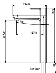
SG-3029PCL2 Pillar Cock Extension Body 10" with Brass Handel & Flange
