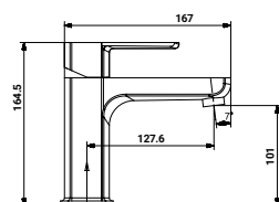
SG-3026SBM Single Lever Basin Mixture with 450mm Tube with Brass Handel & Flange
