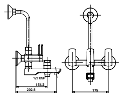
SG-3017WM3 Wall Mixture 3 in 1 with Provision for Over Head Shower with Brass Handel & Flange
