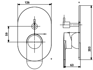
ST-3138SPK2 Exposed Part Kit of Single Leaver Hi/Flow Diverter 45MM with Brass Handel & Flange
