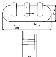
SG-3031DV4 Exposed Part Kit of 4 Way Diverter with Brass Handel & Flange
