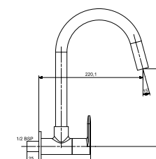
ST-3111SCL Sink Cock Extension Spout with Brass Handel & Flange
