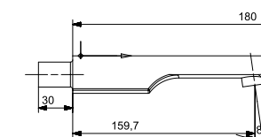
SG-115BTS Bath Tub Spout with Brass Flange
