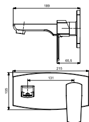
SG-3019SPK Exposed Part Kit of Sink Mixture Wall Mounted Swing Spout with Brass Handel & Flange
