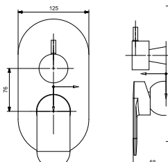
ST-3135SJM Exposed Part Kit of Jet Single Lever 3 Way Diverter (20MM)
