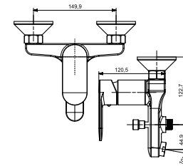
ST-3139SWM Single Lever Wall Mixture with Provision Hand Shower (Wall Mounted) with Brass Handel & Flange
