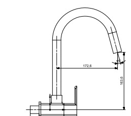
SG-3011SCL Sink Cock Extension Spout with Brass Handel & Flange
