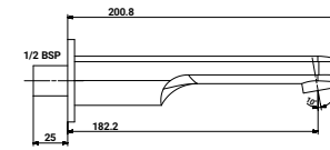
ST-117BTS Bath Tub Spout with Brass Flange
