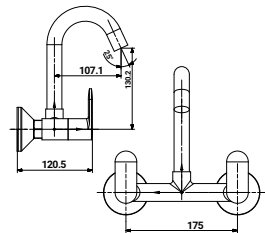
ST-3125LB Long Body Bib Cock with Brass Handel & Flange
